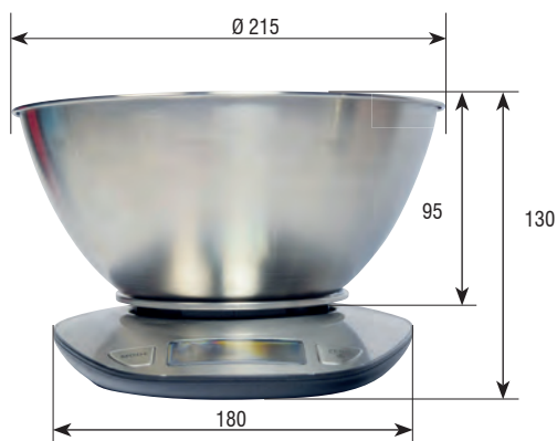
Dimensions (mm)
